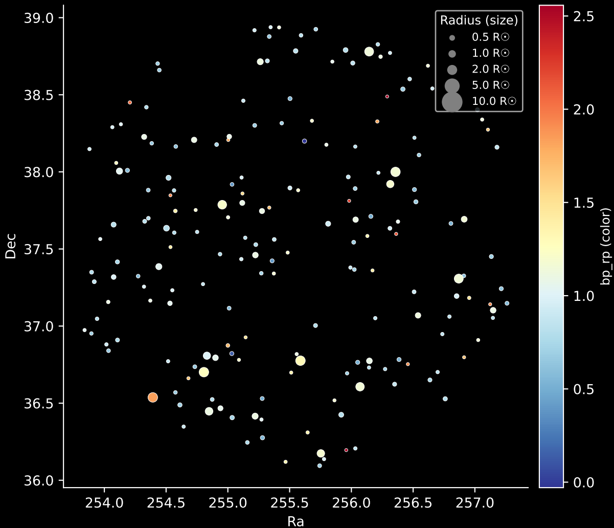
APOGEE DR17 Field: [185+57_MGA] Stars: 192
