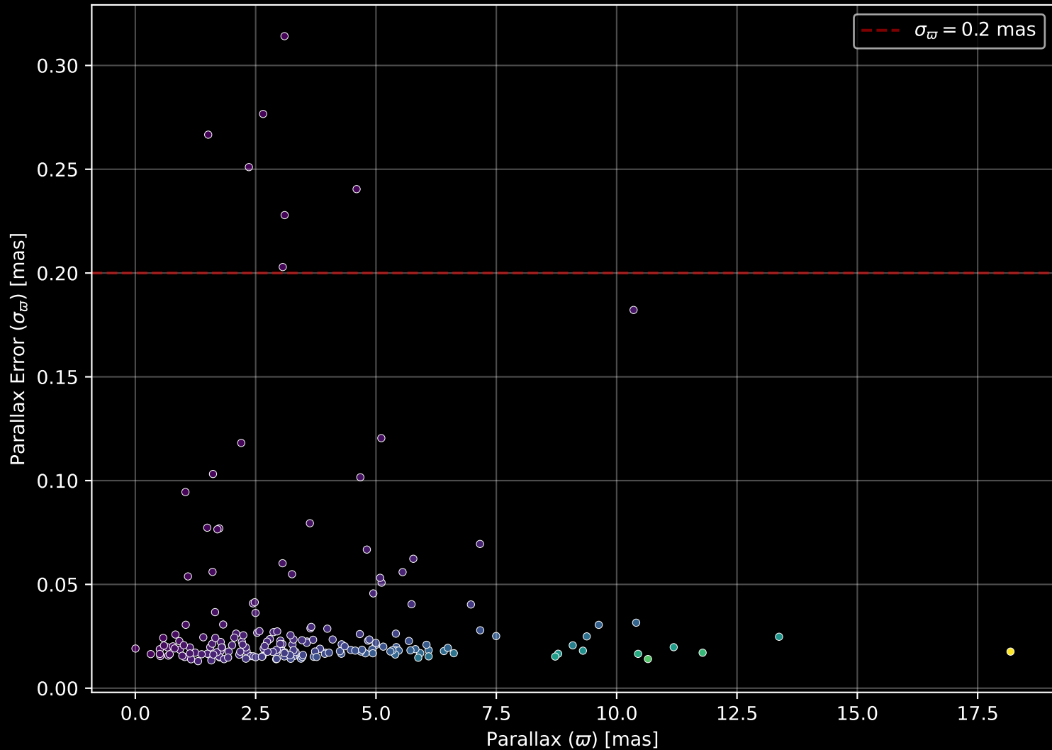
APOGEE DR17 Field: [185+57_MGA] Parallax Quality (n= 192)
