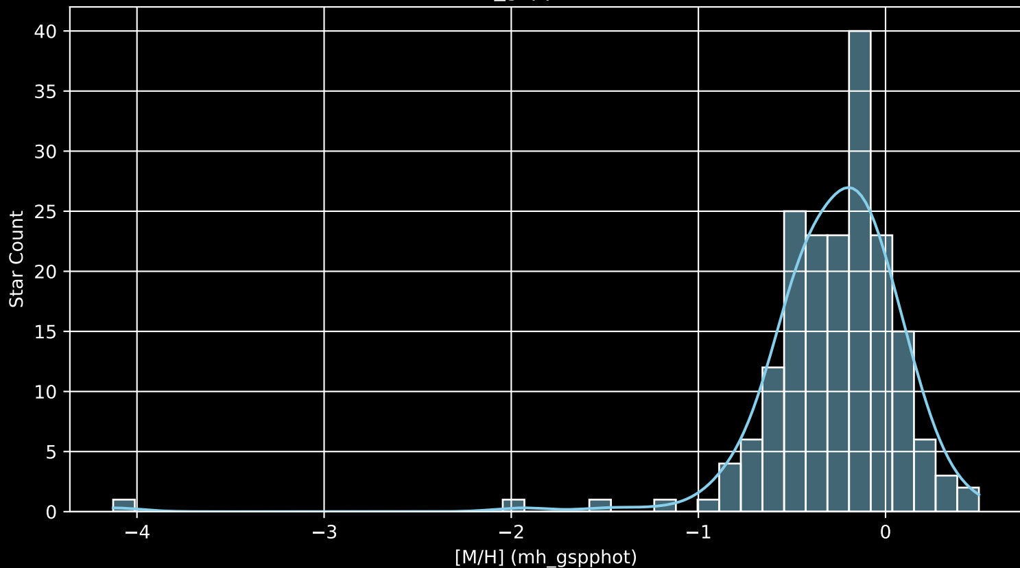
APOGEE DR17 Field: [185+57_MGA [M/H] (mh_gspphot) (n= 187)
