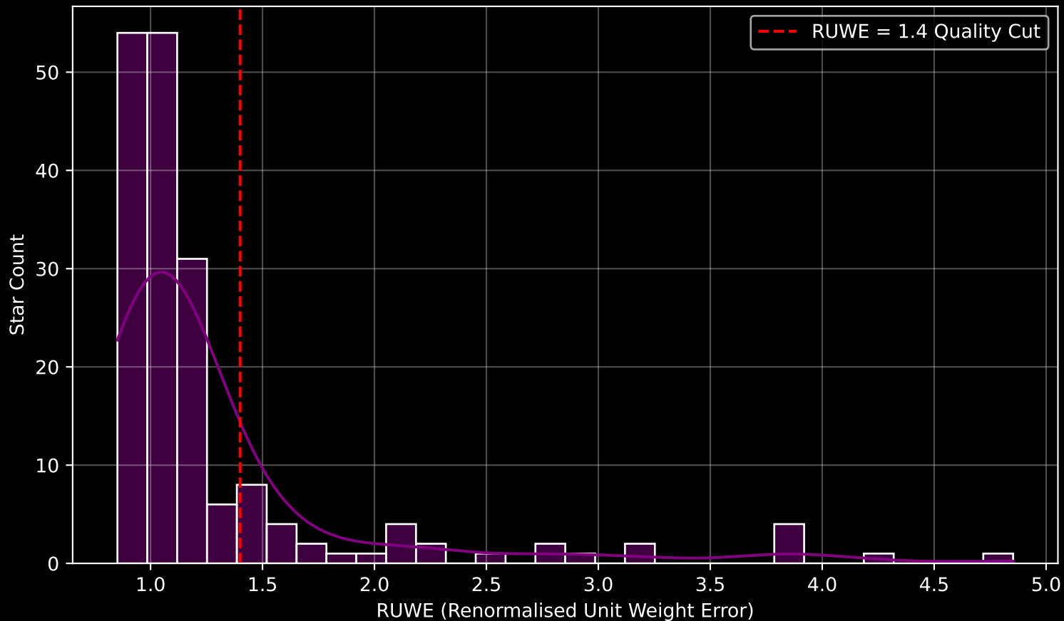
GAPOGEE DR17 Field [185+57_MGA] RUWE Distribution (n= 179)
