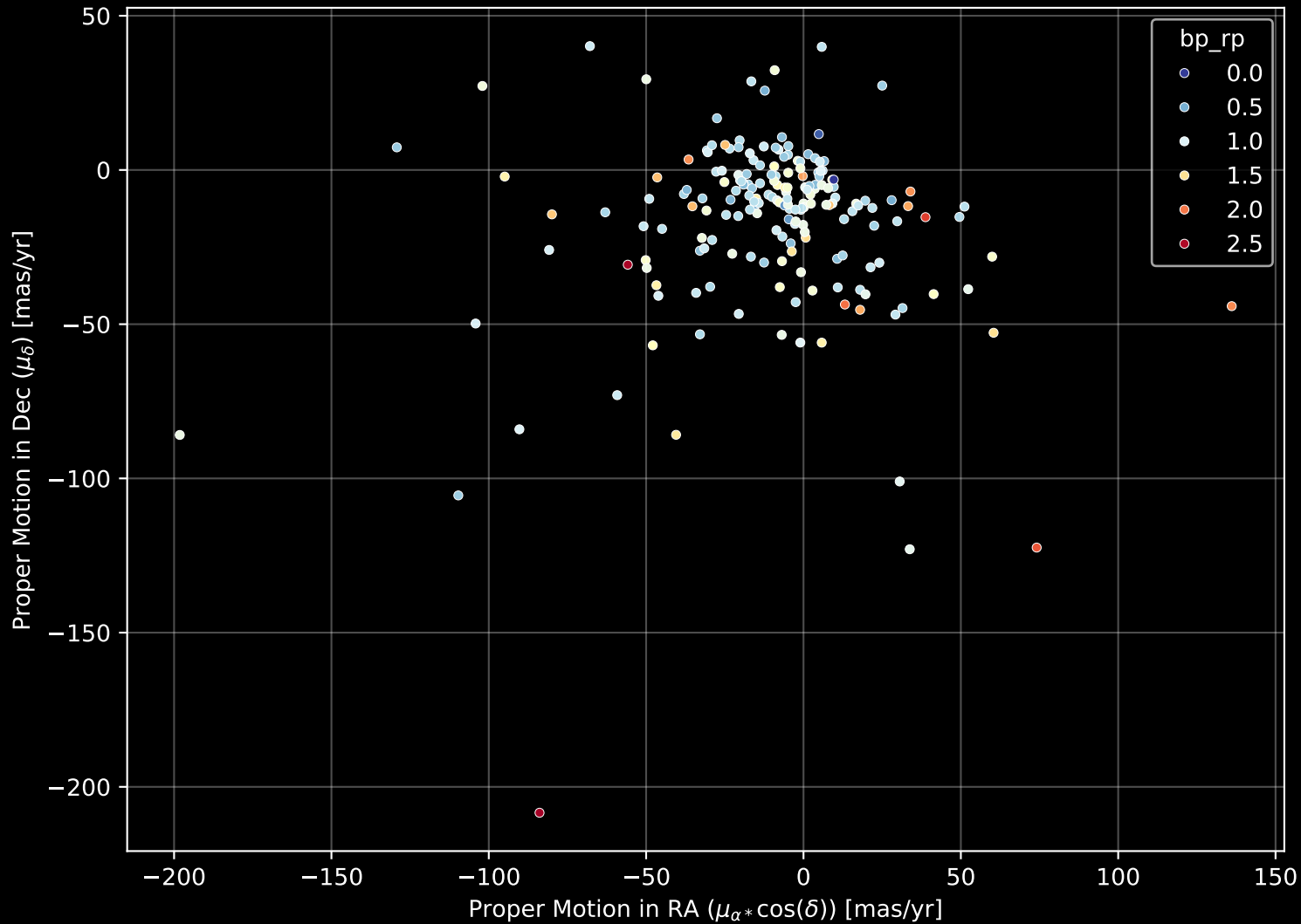
APOGEE DR17 Field: [185+57_MGA] Proper Motion Diagram (n= 192)
