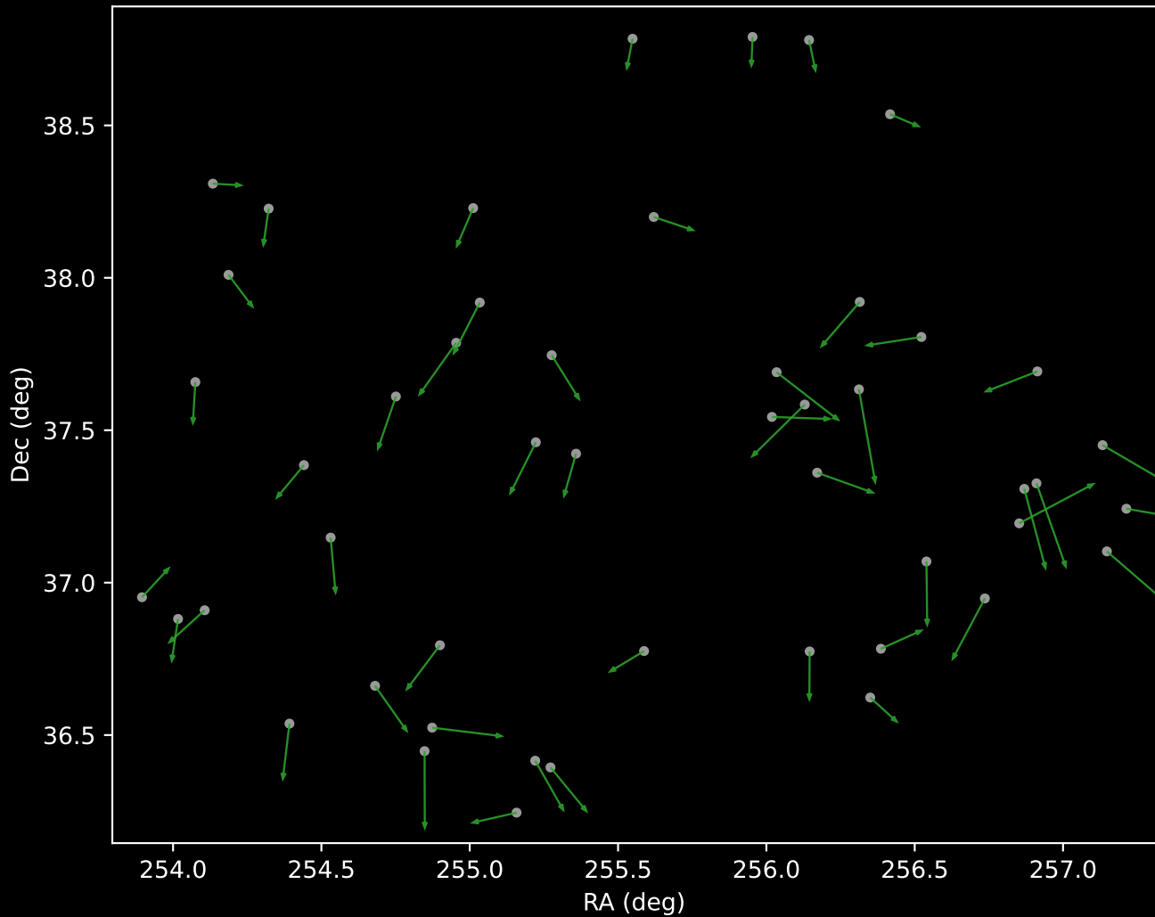
APOGEE DR17 Cluster 4 Proper Motion Vectors (n=49)
