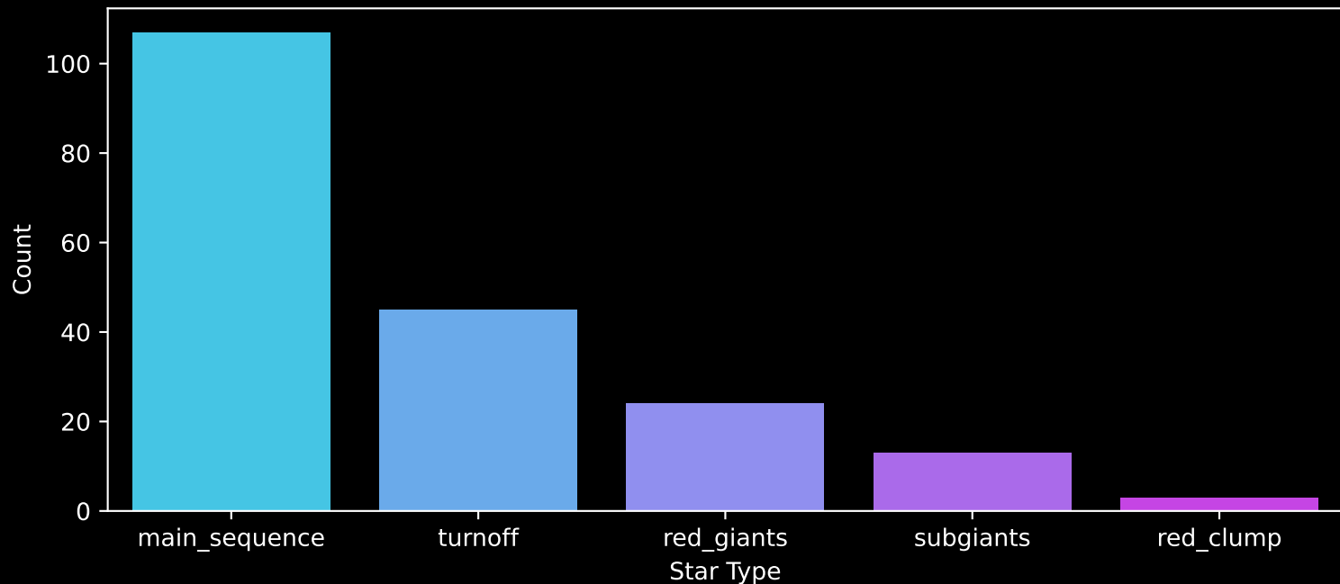
APOGEE DR17 Field: [185+57_MGA] Count plot of Star Type
